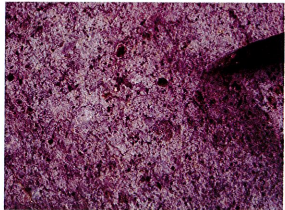
Figure 3. Granitic rock from Lalang island (Sembilan group). The main rock type is coarse to medium-grained equigranular biotite granite. Note that the granitic rock from Lalang island is leucocratic compared to the Jarak granite.
