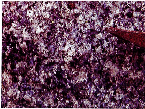
Figure 2. Coarse to medium grained equigranular biotite granite of the Jarak island. Note the bluish colour of the quartz crystal.
