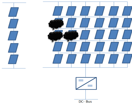
Figure2 Proposed PV system configuration with adaptive and fixed parts central DC/DC converter
