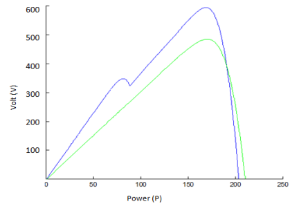
Figure 3 PV characteristic before recovering with mismatch conditions
