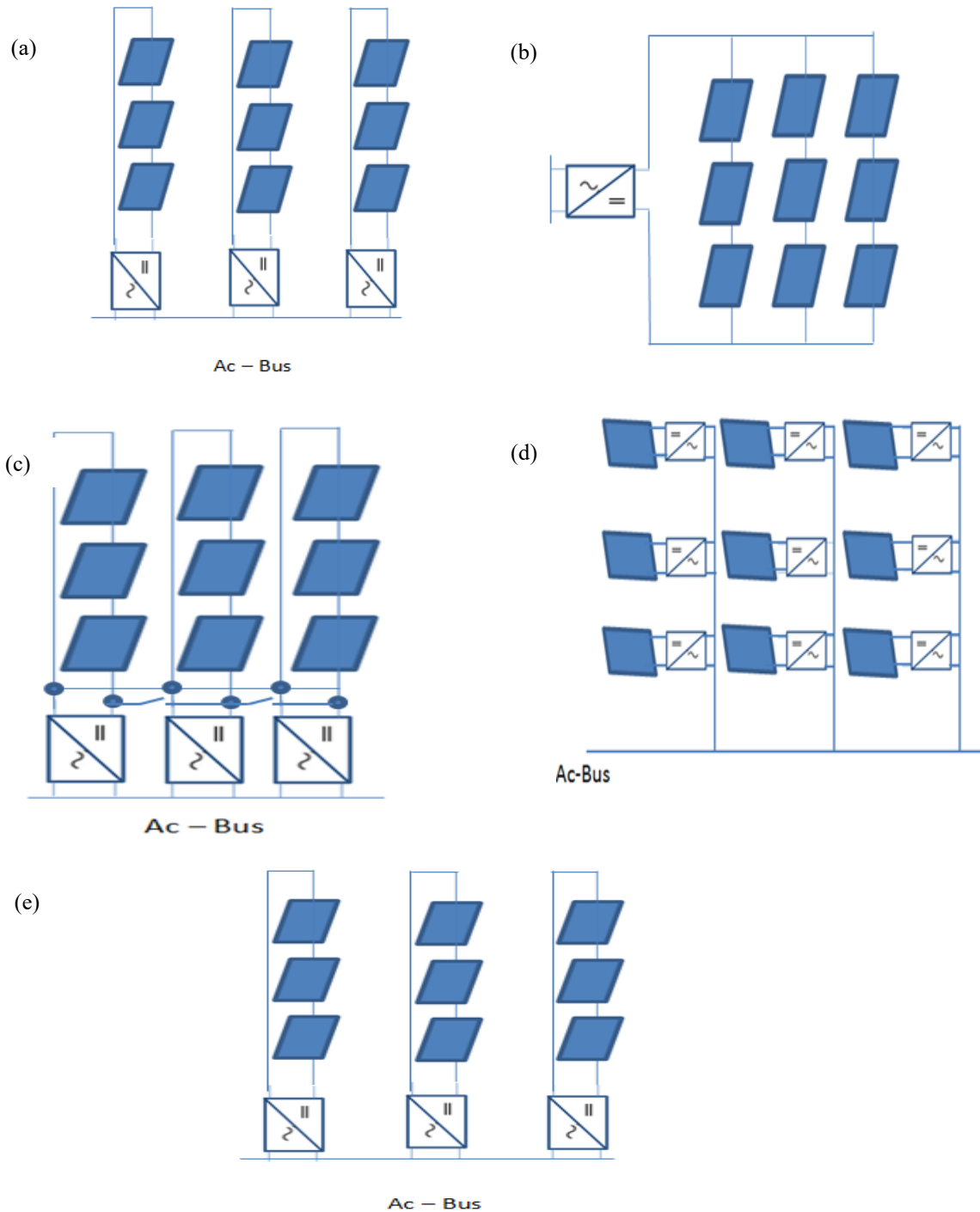
(a)The configuration of string inverter, (b) The configuration of central inverter, (c) The configuration of team inverter, (d) The configuration of modular inverter, (e)The configuration of multi DC-DC central inverter.
