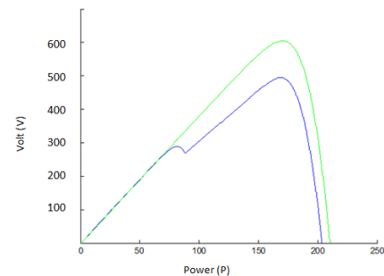
Figure 4 PV characteristic after recovering with mismatch conditions
